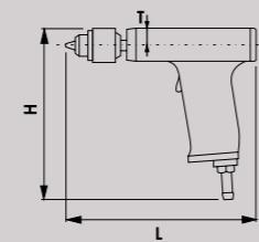
Models PV (without hose)
